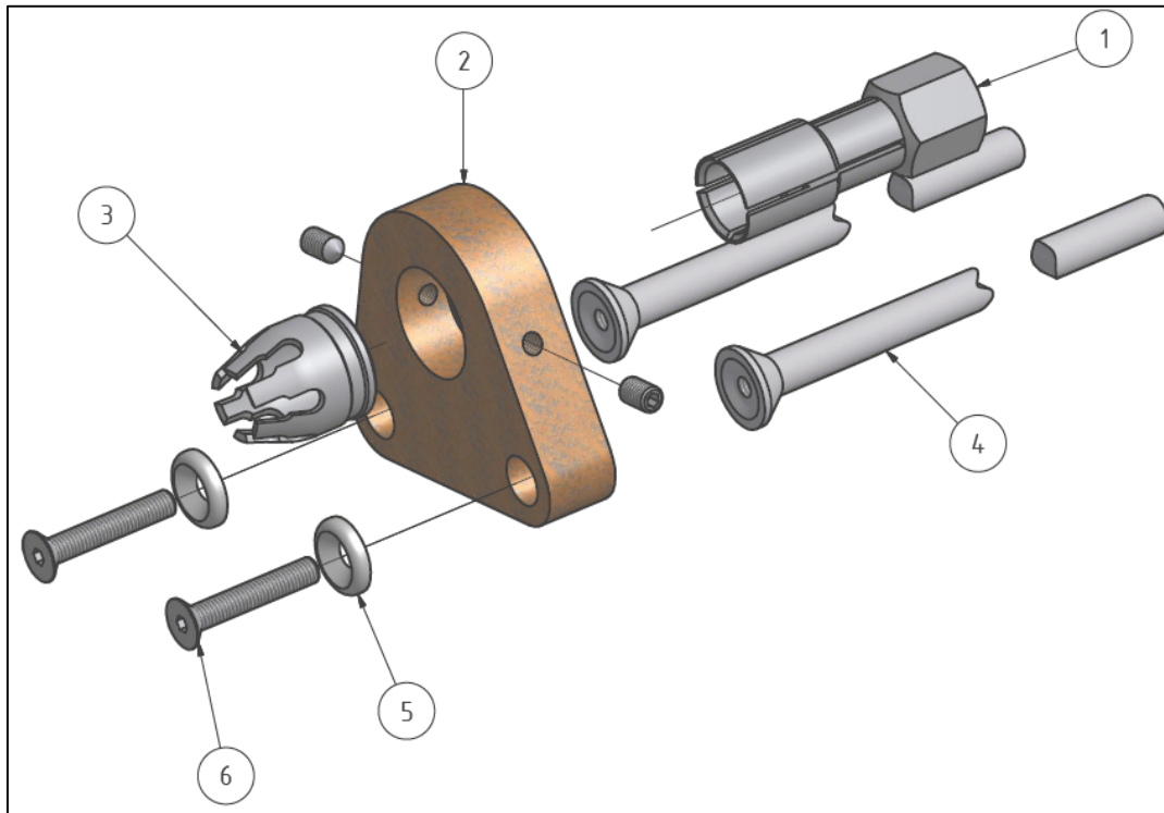
Figure 44: Gun accessories for threaded studs, tapped studs and plain pins
