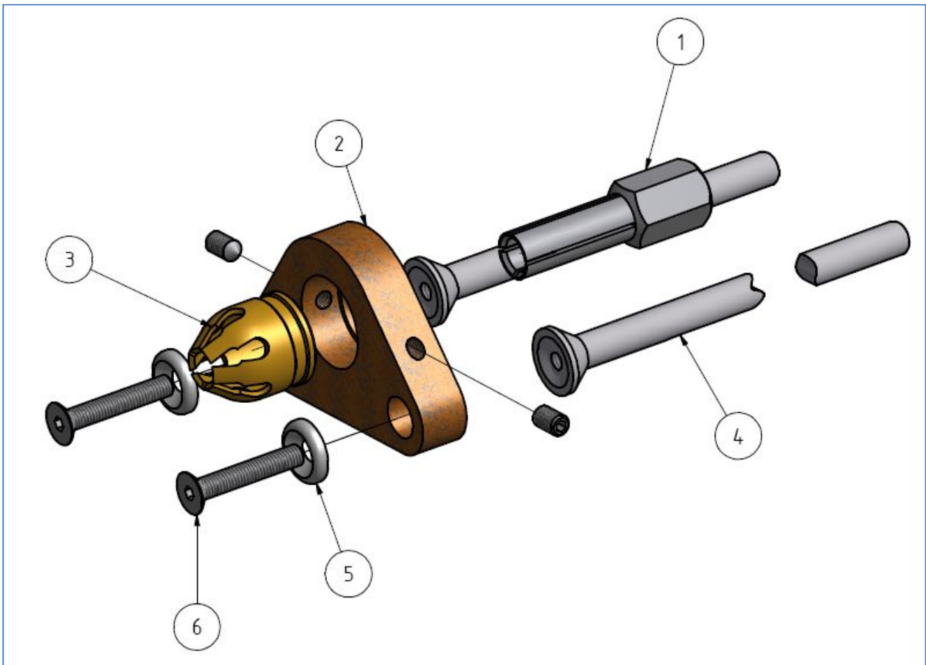
Figure 30: Gun accessories for threaded studs and plain pins
